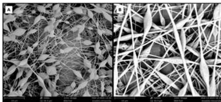
Figure 6. SEM images of the samples at different PMMA molecular weight: 81.000 MW (A),350.000 MW (B) .
