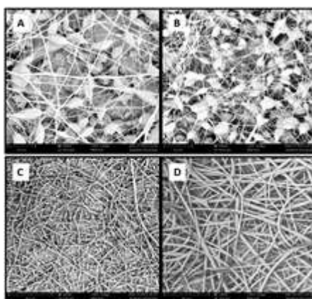
Figure 8. SEM images of the samples under the effect of Silane additives (A) pure PMMA/BNNS nanofiber (81.000 g/mole PMMA) (B) with silane additives PMMA/BNNS nanofiber (81.000 g/mole PMMA) (C) pure PMMA/BNNS nanofiber (350.000 g/mole PMMA) (D) with silane additives (350.000 g/mole PMMA)
