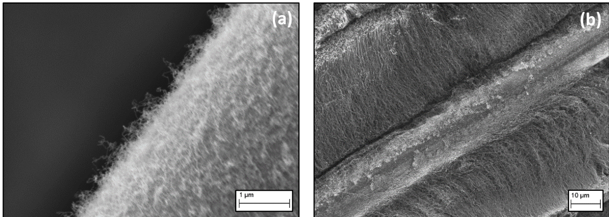
Figure 4. Carbon nanotube-grafted-quartz fibres exhibiting; (a) short (ca. 200 nm) and (b) long (ca. 20 \mu\text{m} ) carbon nanotube growth.
