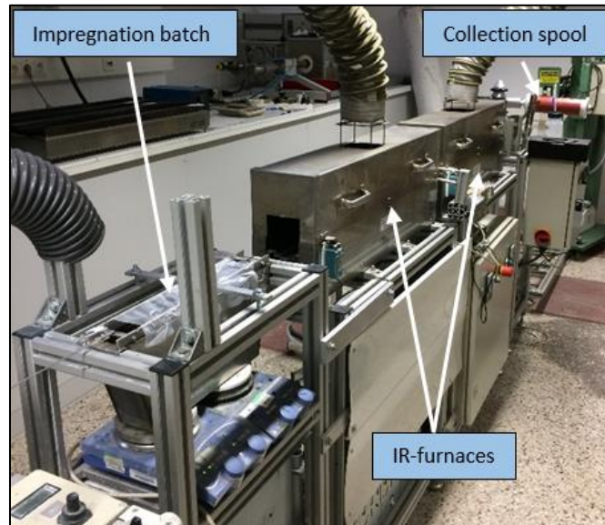
Figure 1. Photograph of the catalyst precursor deposition line.
