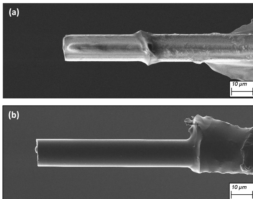
Figure 6. Scanning electron microscope of (a) CNT-grafted-quartz fibre (short) and (b) CNT-grafted-quartz fibre (long) fracture surface after pull-out.
