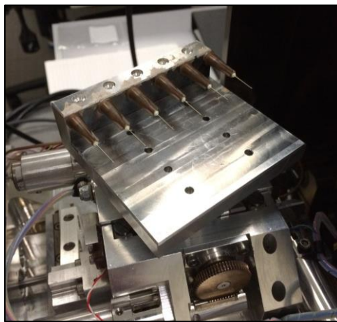
Figure 5. Photograph of single fibre pull out specimen holder for scanning electron microscopy.
