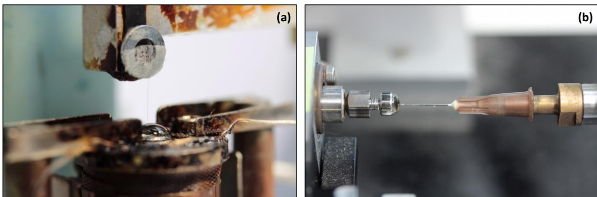
Figure 3. Photographs of (a) the fibre embedding kit and (b) the single fibre pull out set-up.
